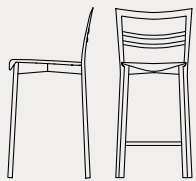
CB1689 43x49 H94 HS65 cm
